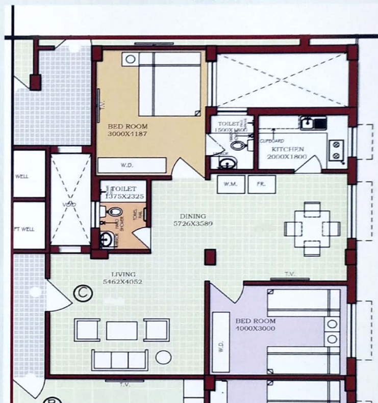
Floor Plan
