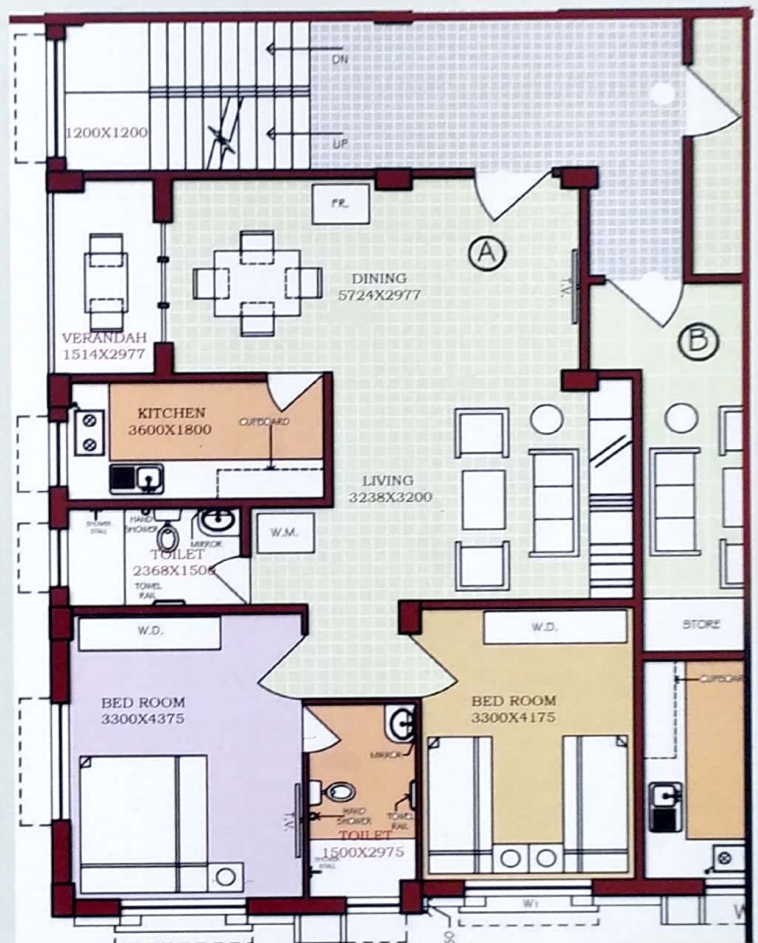
Floor Plan
